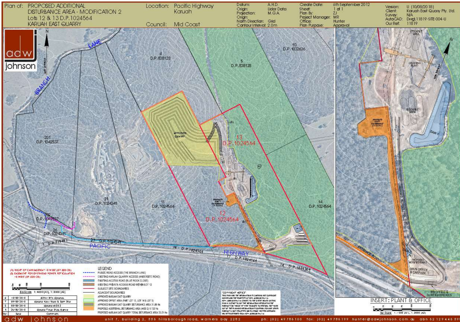
Figure 1: Development Layout
