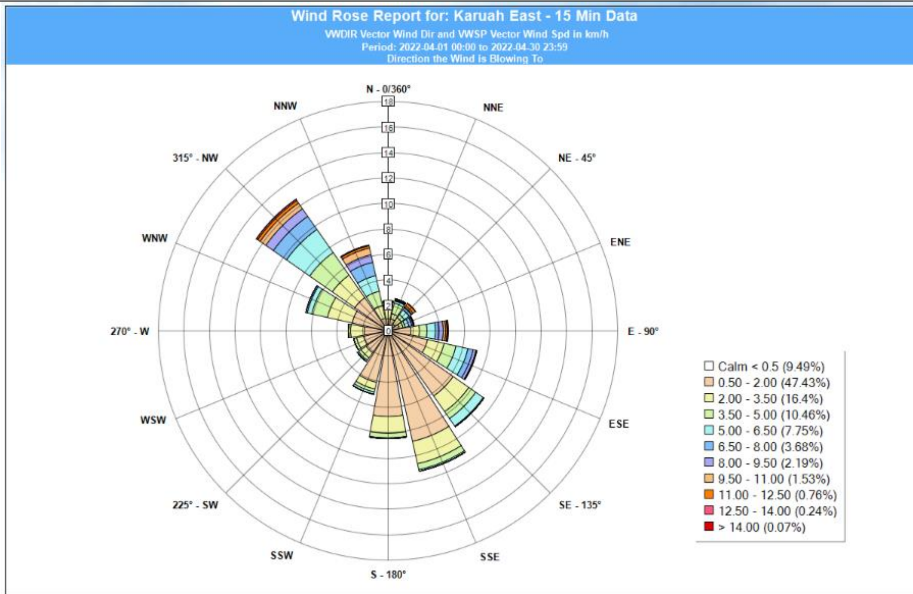
Figure 3 Wind rose April 2022
