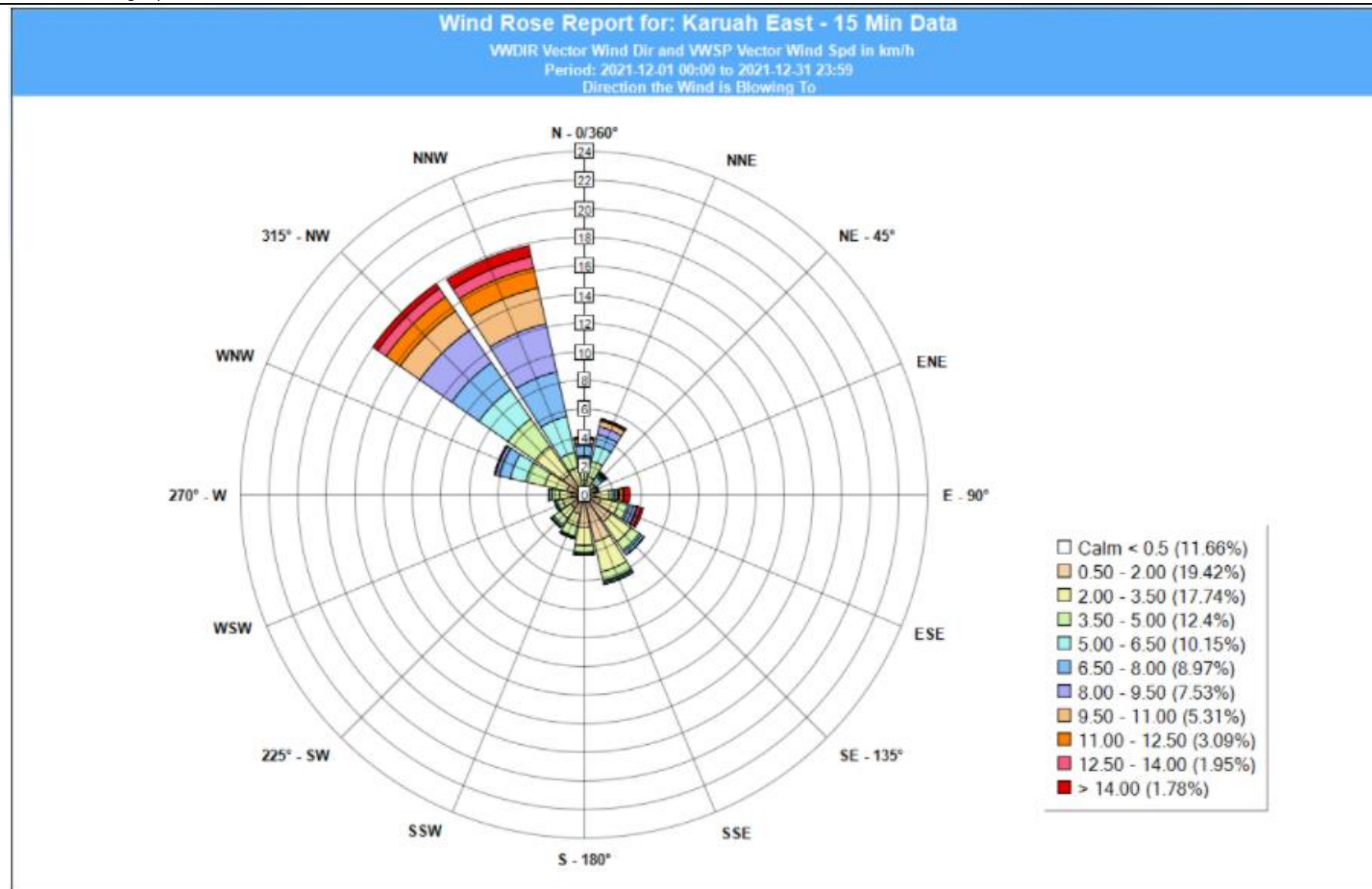
Figure 3 Wind rose December 2021
